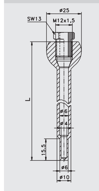
Tuleja wspawana do L=150, ESH-KM12/...-06
