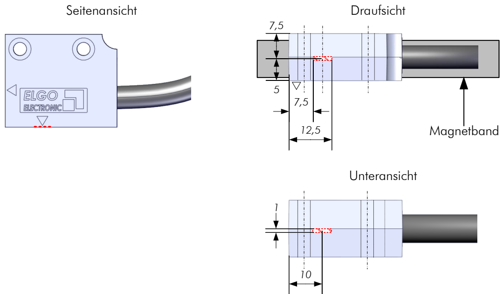
Abbildung 6: Horizontale Sensorposition (Standard)
