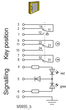
Fig. 1: Locked while activated: Key inserted
