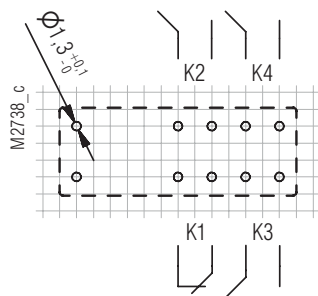
OA5670.48__L1 3NO/1NC
