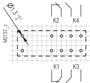
OA5670.52__L1 2NO/2NC
