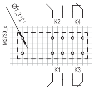
OA5670.52__L2 2NO/2NC
