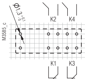
OA5670.52__L3 2NO/2NC
