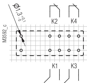
OA5670.52__L4 2NO/2NC
