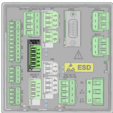
DC ±5 V: OUT 8/9
