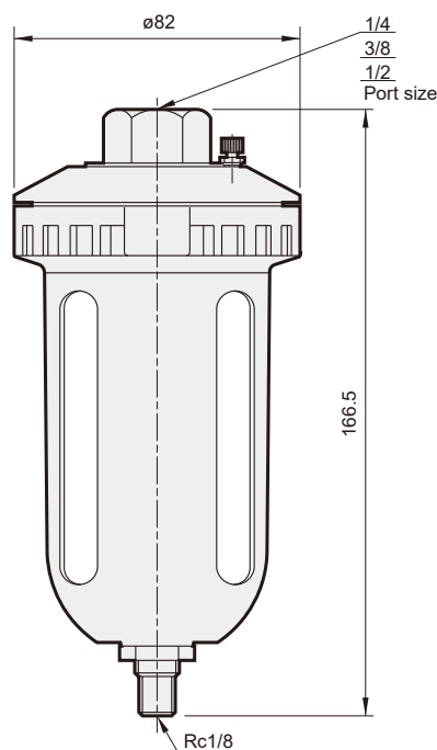
MAD400 Male thread (MADV400-WB)
